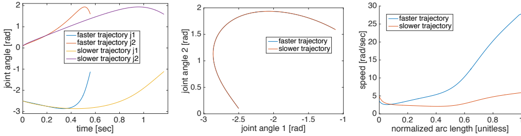
Figure 1: Trajectory representation with AL-DMPs. Left: trajectories of movement of a robot with two degrees of freedom, executed at two different speeds. The result are spatially identical but temporally different movements. The faster movement was generated by nonlinear scaling of the slower movement (its speed was multiplied by a factor of 2(t+1)e^{(t+1)^2-2} , t \in [0, T] , T = 0.5345 , T is the duration of the faster movement). The consequence of nonlinear scaling is that the spatial parameters \mathbf{w} in the DMP forcing term change. Middle: the reproduction of the spatial course of movement by AL-DMP. Since arc-length derivatives are independent of speed, in AL-DMP the weights \mathbf{w} do not change and consequently the spatial courses of the two movements are identical. Right: Speed s of both movements as a function of normalized arc-length, i. e. s/L . As shown in the graph, the speed change is nonlinear and cannot be reproduced by linear scaling of the standard DMP, i. e. changing the parameter \tau .
