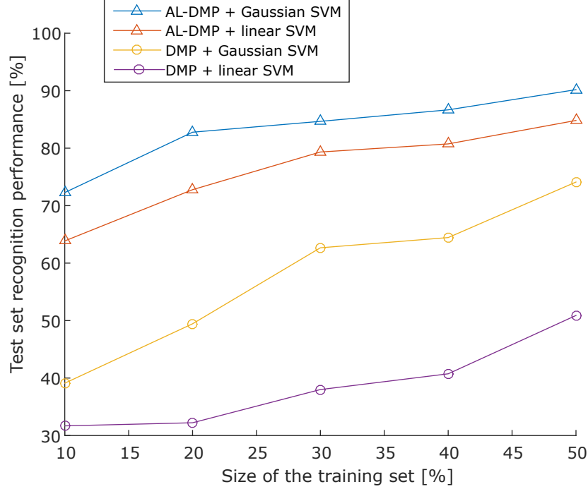
Figure 10: Classification performance as a function of the training set size. Blue and red graphs show the percentage of correctly classified examples using the Gaussian and linear SVM, respectively, with AL-DMP weights used as features. Yellow and magenta show classification performance when standard DMP weights were used as features.
