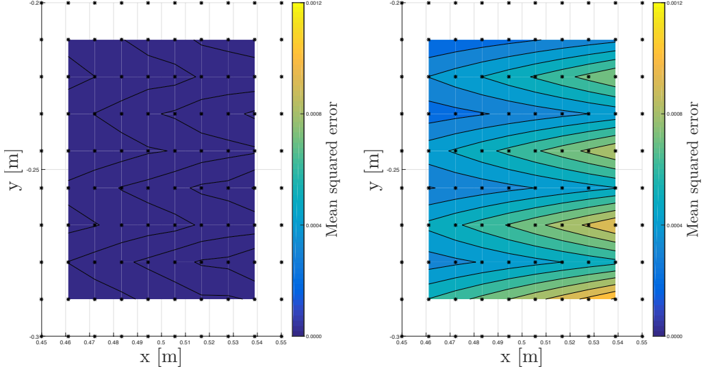
Figure 4: Contour plots showing the accuracy of generalization with AL-DMPs (left) and DMPs (right) in simulation. Generalization with AL-DMPs is clearly better.
