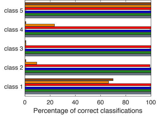
Figure 9: Classification performance for simulated reaching movements. The grey, green and blue bars show the classification performance of AL-DMPs, DMPs, and B-splines using the original data, while the red, orange and brown bars show the classification performance of AL-DMPs, DMPs, and B-splines using temporally scaled data.
