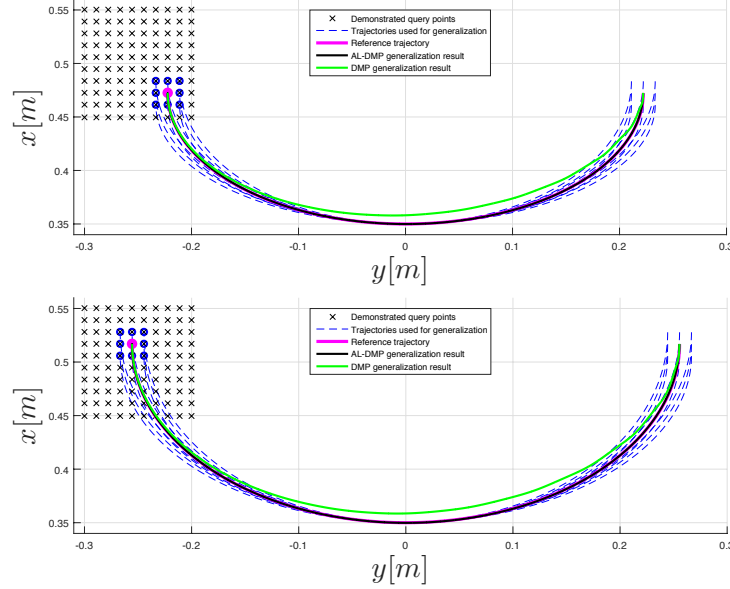
Figure 3: Two example generalizations in 2-D plane using AL-DMPs and standard DMPs. The original trajectories that were used for generalization are shown in blue and dashed. They all pass through a unique via point at y = 0 . The trajectories generalized using AL-DMPs (black) also pass through this via point. The trajectories generalized using DMPs (green) do not approximate the original trajectories well and do not pass through the via point.
