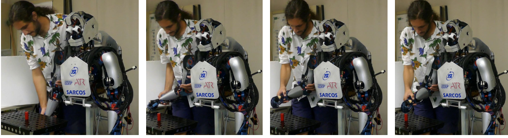
Figure 2: Teaching of humanoid reaching trajectories by kinesthetic guiding from the initial configuration (left) to the final reaching position (right).
